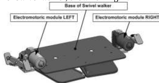
Fig. 2. Swivel Walker with electromotoric module
