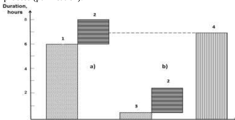
Figure 1 - Duration of technological operations wastewater treatment using coagulant by traditional (a) and Express method (b) of control 1 - Control of suspended solids by traditional method; 2 - The process of coagulation; 3 - Control of suspended solids through transparency of wastewater; 4 - Finding of wastewater on purification station Slavutych town
