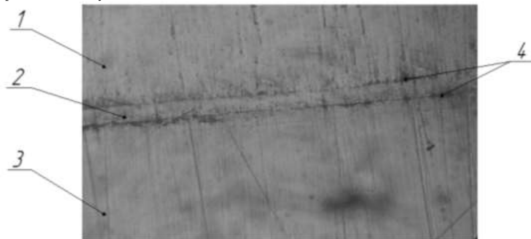
1 – copper; 2 – porous nickel; 3 – bismuth telluride; 4 – indium;
