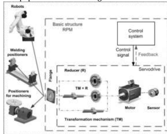
Fig. 1 Deployment of RPM in machinery and equipment
