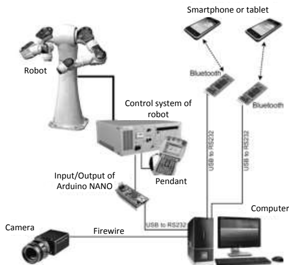
Fig. 1 Interconnection devices
