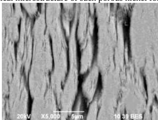
Fig.1. The microstructure of nickel foil, that was made by the method of electron-beam evaporation and deposition from the vapor phase in vacuum [7]
